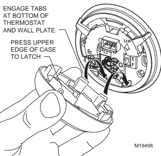
Fig. 9. Mounting thermostat to wallplate.
